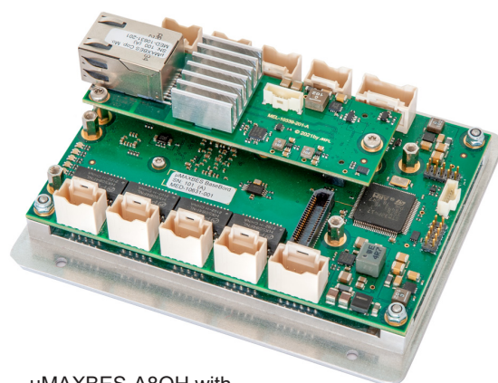
μMAXBES-A8OH with 1x 10Gbit copper port (1x μMAXBES-RJ1)
