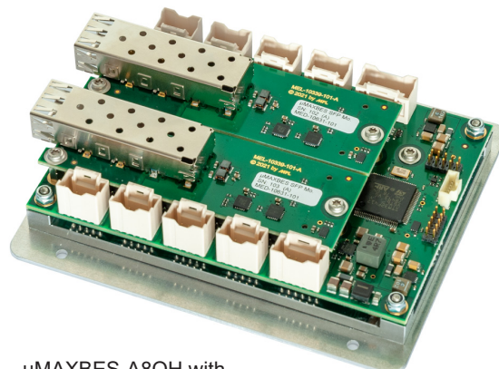
μMAXBES-A8OH with 2x 10Gbit fiber ports (2x μMAXBES-SFP1)
